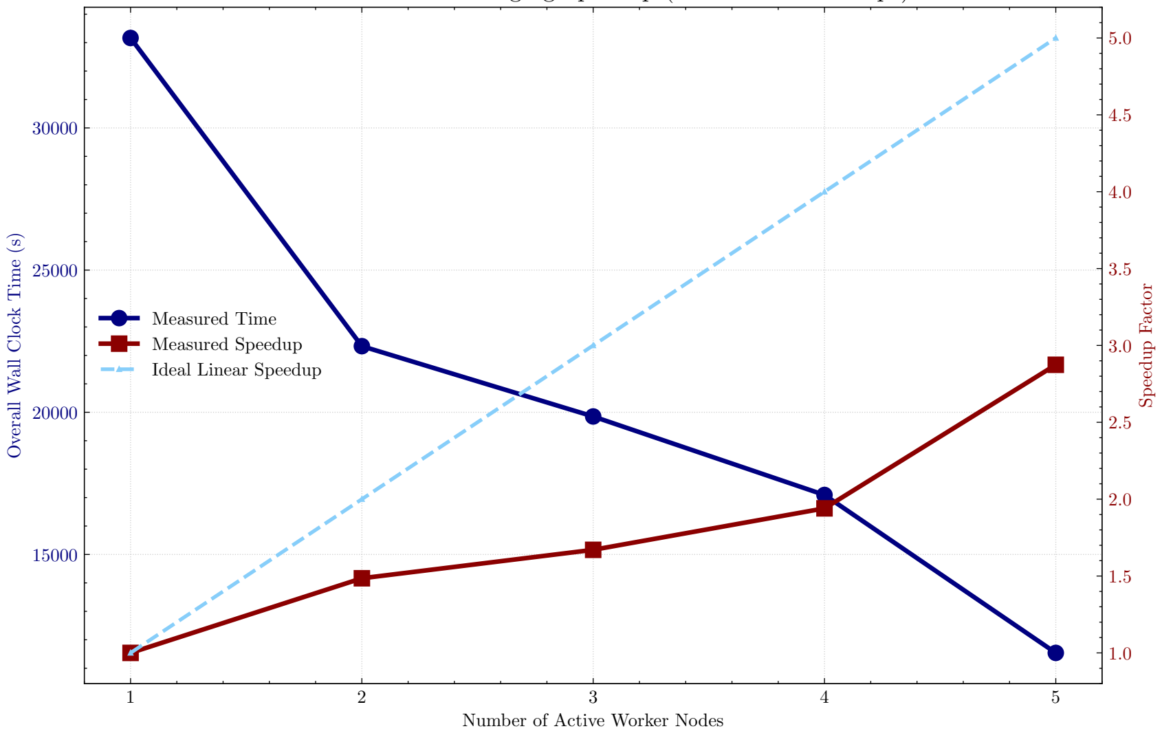
MPI Ensemble Averaging Speedup (10 Million MC Steps)
