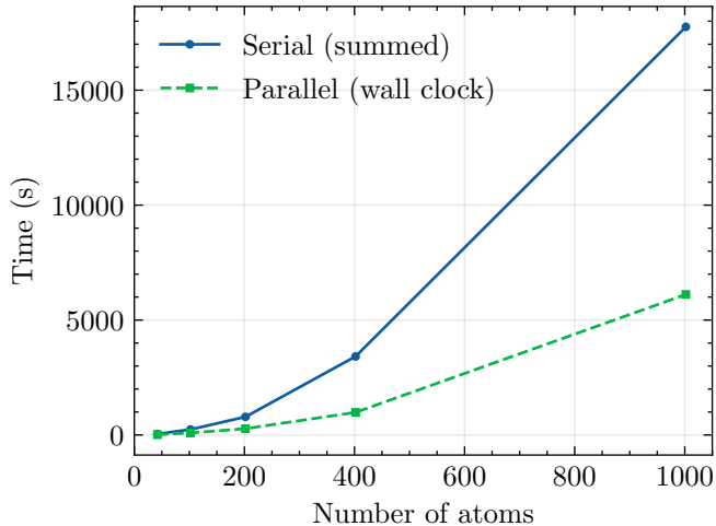
Wall time vs N_{atoms} ( n_{steps} = 10^6 )
