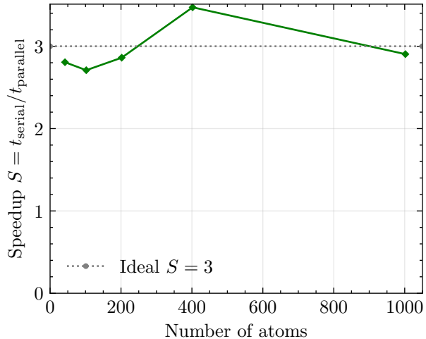
Speedup vs N_{atoms} ( n_{steps} = 10^6 )
