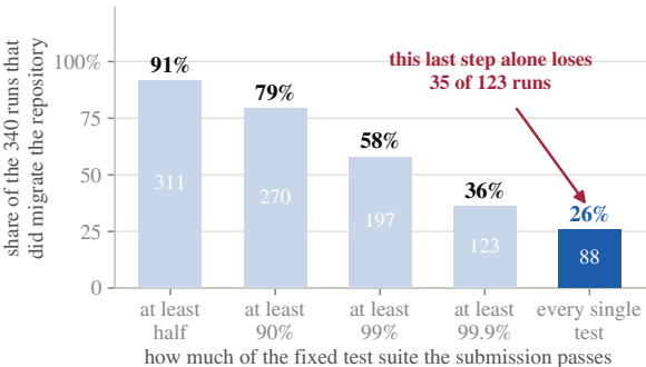
(a) Reaching 99% is common; reaching 100% is not
