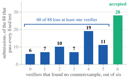
(b) 100% on the tests is still not enough
