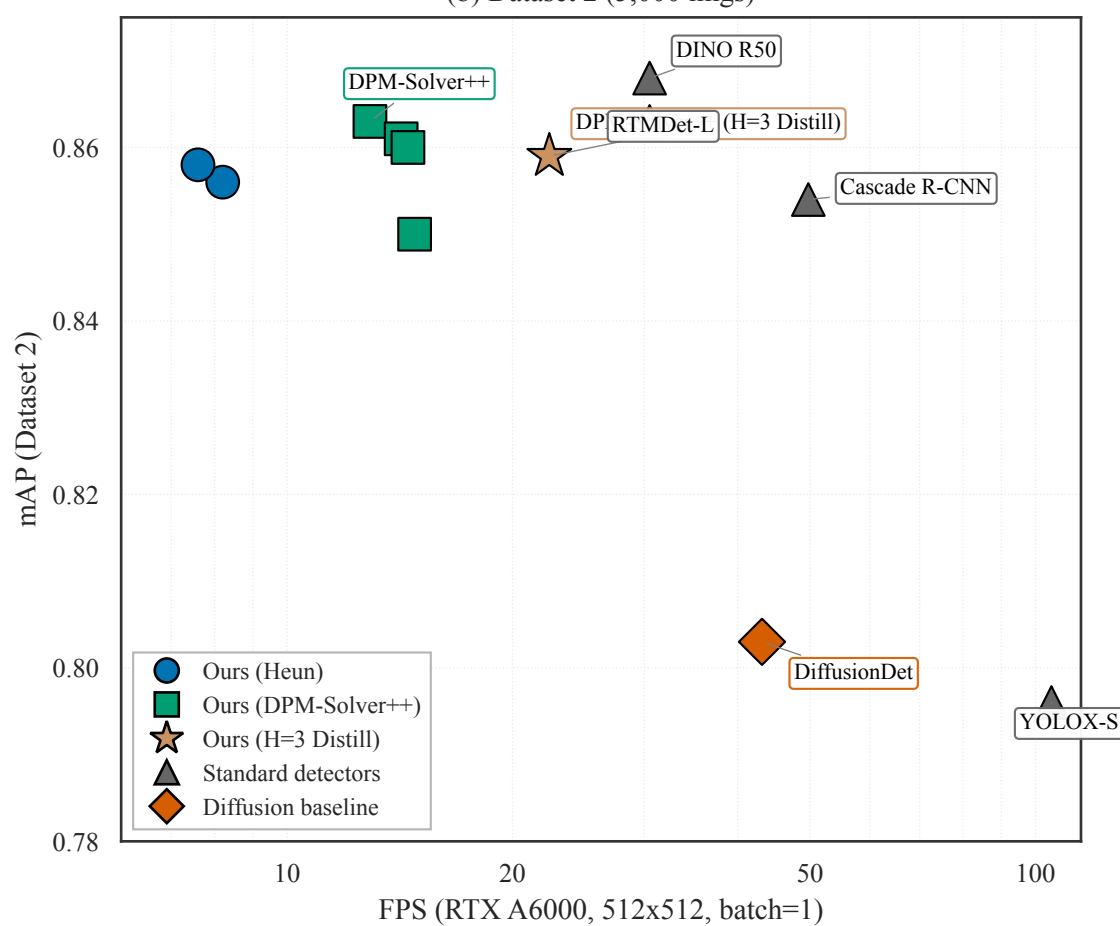
(b) Dataset 2 (5,000 imgs)
