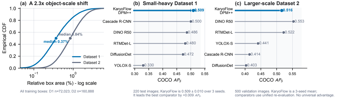
Fig. 5. Object-scale shift and small-object detection across two chromosome cohorts. (a) Empirical CDF of relative ground-truth box area using all training annotations. Dataset 1 boxes are markedly smaller than Dataset 2 boxes. (b) Dataset 1 test AP S on 220 images; KaryoFlow is the clean random-coupling three-seed mean and leads the strongest listed comparator by 0.0090. (c) Dataset 2 validation AP S on 500 images; KaryoFlow is the three-seed mean and the other detectors use the unified checkpoint-linked re-evaluation. It is competitive but does not lead DINO R50 or RTMDet-L. AP S is interpreted within, not across, datasets.
