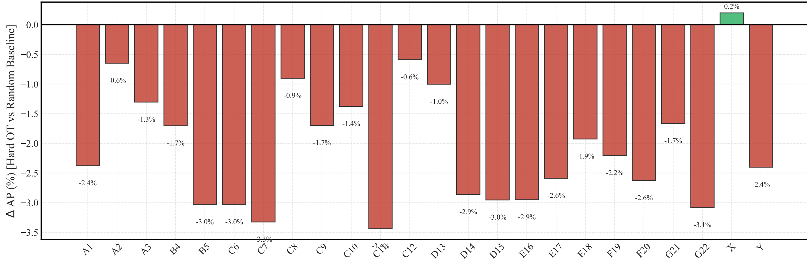
Systematic Performance Degradation Across 24 Chromosome Classes (Hard OT)
