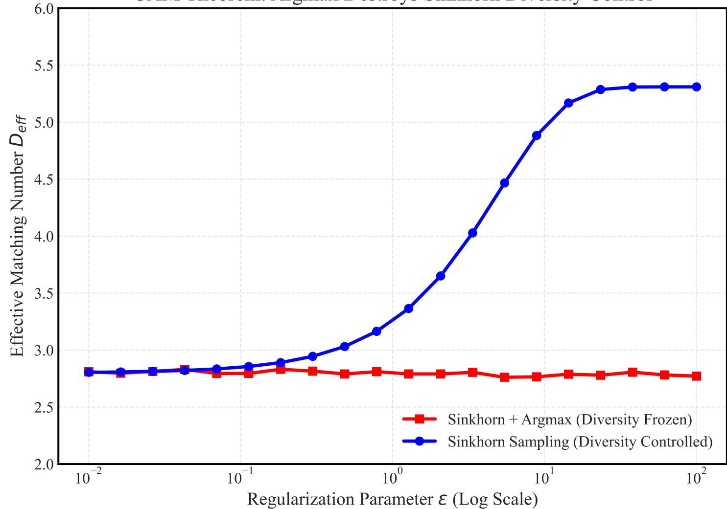
CAM Theorem: Argmax Destroys Sinkhorn Diversity Control
