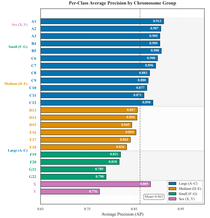
Fig. 6. Per-class AP on Dataset 2 validation (A3 DPM-Solver++). Bars colored by chromosome size group; dashed line = overall mean. Large (A–C) chromosomes achieve highest AP; small (F–G) and Y lowest. Y is the hardest class due to data scarcity and biological variability.
