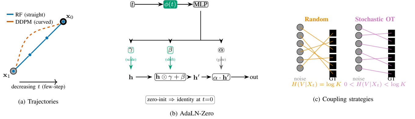
Fig. 1. KaryoFlow overview. (a) RF replaces the curved DDPM trajectory with a straight-line ODE path from noise x_1 to GT box x_0 ; nodes = 4 solver steps. (b) Time conditioning via AdaLN-Zero zero-initialized modulation (identity at t=0 ). (c) Coupling: Random pairing (orange) keeps full diversity H(V|X_t) = \log K ; Sinkhorn-based Stochastic OT (pink) interpolates between hard OT and Random ( 0 < H < \log K ).
