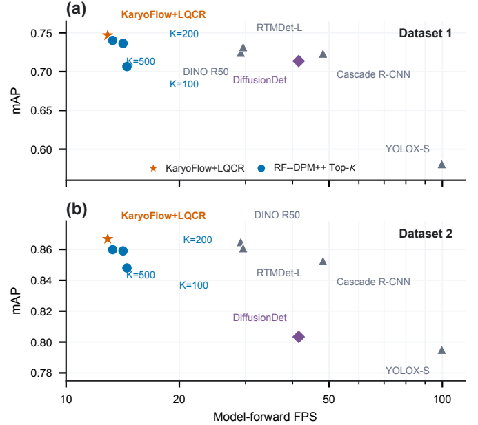
Fig. 1. Fixed-model deployment operating points on two chromosome cohorts. Model-forward FPS is measured with the same 512 \times 512 , batch-1 RTX A6000 protocol. Accuracy points in both panels are three-inference-seed means from fixed trained models. Both panels include three unconnected RF-DPM++ operating points at K = 500, 200 , and 100 ; the Dataset 1 K = 200/100 points use inference-only pruning of the same model. The star denotes the full KaryoFlow+LQCR operating point; circles denote RF-DPM++ Top- K settings. Independent-training estimates are reported in Table V. Higher and farther right is better.
