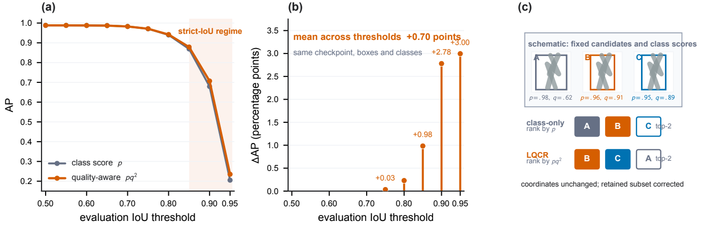
Fig. 3. Effect and operating scope of localization-quality ranking. (a) On the same Dataset 2 RF-DPM++ model, quality-aware and class-only AP curves separate mainly at strict IoU thresholds. (b) Their threshold-wise difference reaches +2.78/+3.00 points at AP90/AP95, while AP50 changes by only −0.01 percentage points. (c) A schematic keeps candidate boxes and class scores fixed before class-only and LQCR ranking; localization quality promotes the tighter candidate and changes the retained top-2 subset without altering candidate geometry. Panels (a)–(b) report held-out measurements; (c) illustrates the ranking mechanism.
