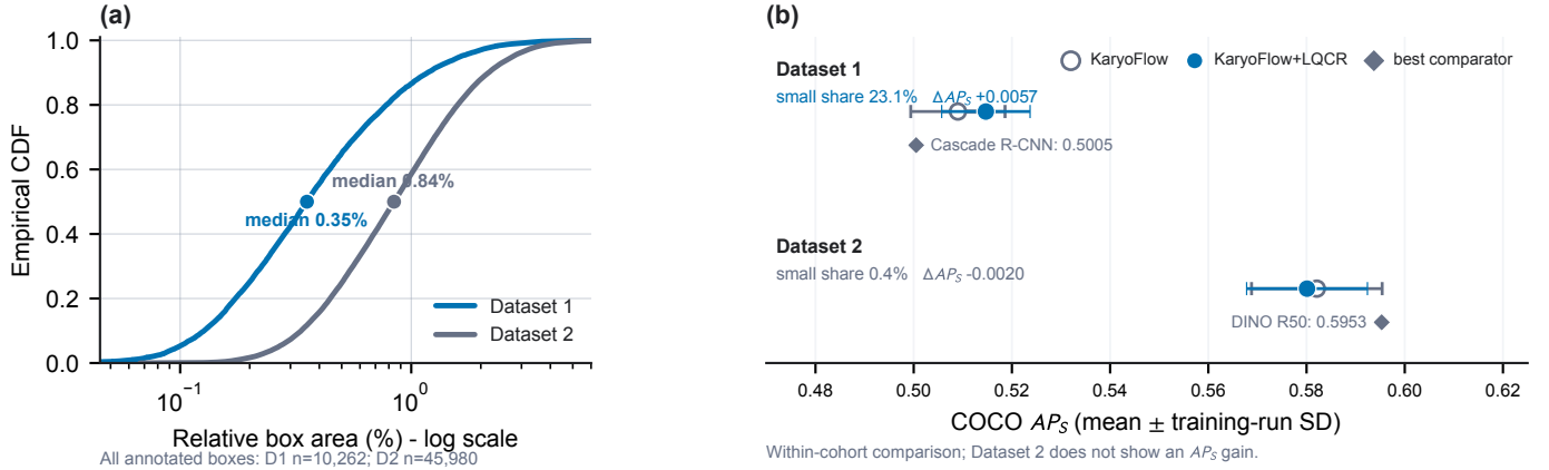
Fig. 4. Object-scale shift and scale-resolved detection across two chromosome cohorts. (a) The empirical CDF of relative ground-truth box area over all test annotations shows that Dataset 1 chromosomes are markedly smaller than those in Dataset 2. (b) Paired point-and-interval summaries show the KaryoFlow and KaryoFlow+LQCR AP_S means and training-run SDs; the direction of the LQCR change is explicitly retained for each cohort. AP_S is interpreted within, not across, datasets. Each KaryoFlow estimate uses three independently trained detector pairs; conventional comparators are fixed-model point estimates.
