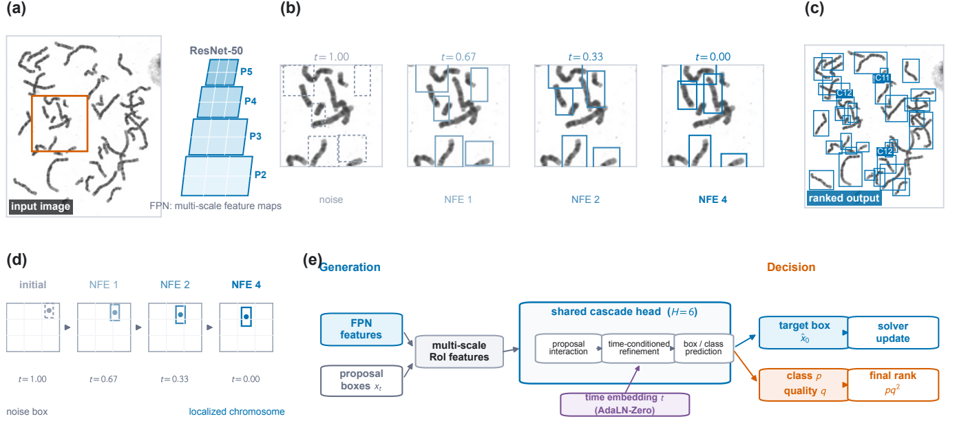
Fig. 2. KaryoFlow from image to detections. (a) A metaphase image and its ResNet-50-FPN representation provide multi-scale image features. (b) A dense crop shows selected snapshots from the prescribed four-NFE box-refinement sequence, from noise to localized chromosome candidates. (c) The detector emits the final quality-ranked chromosome detections. (d) One proposal is shown in normalized center-and-scale coordinates along the prescribed linear RF path. (e) At each evaluation, multi-scale RoI features feed a shared cascade head for proposal interaction, time-conditioned refinement, and box/class prediction; localization quality is used only in the final decision stage. Endpoints and output boxes are empirical; intermediate boxes visualize the prescribed RF path rather than recorded hidden activations.
