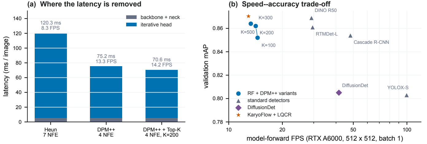
Fig. 4. Same-hardware efficiency on Dataset 2. (a) Latency decomposition. (b) Validation mAP versus FPS on one RTX A6000; connected points form a checkpoint-paired Top- K sweep. The highlighted LQCR point is the complete KaryoFlow accuracy model; other detectors are independent.
