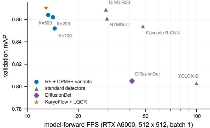
(b) Speed-accuracy trade-off
