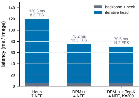
(a) Where the latency is removed
