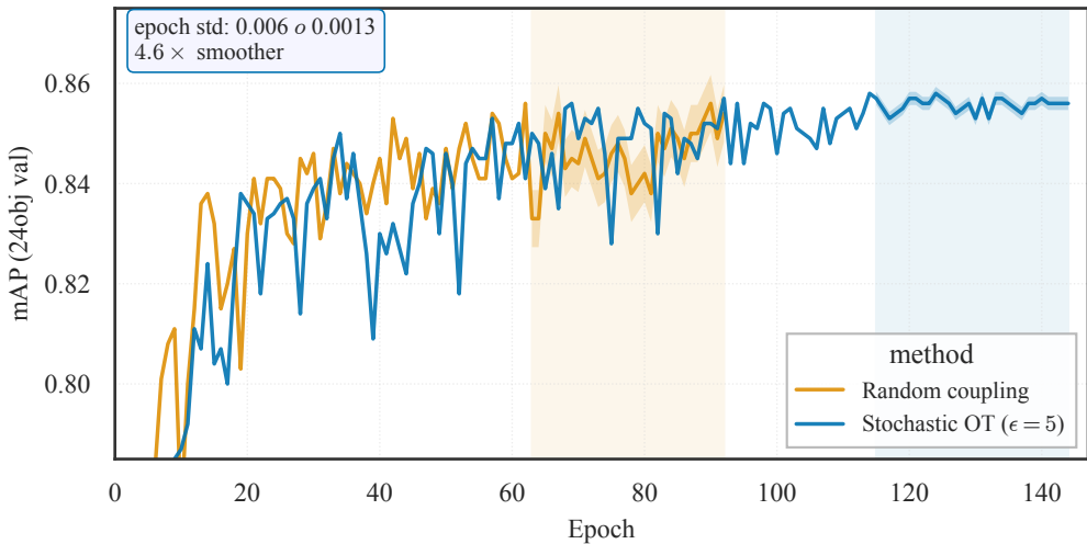
Training Stability: Random vs Stochastic OT
