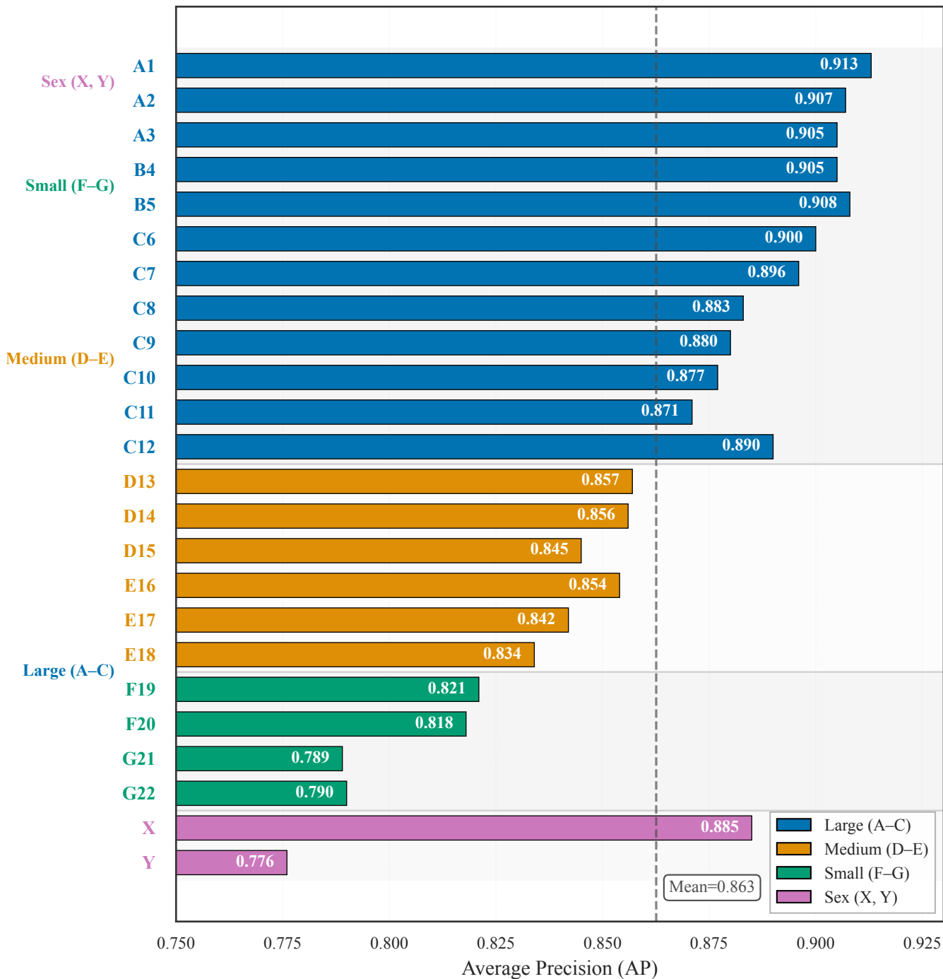
Per-Class Average Precision by Chromosome Group
