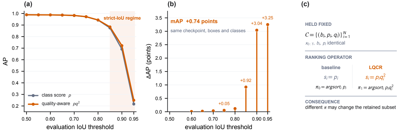
Fig. 2. Effect and causal scope of localization-quality ranking. (a) On the fixed Dataset 2 seed-42 RF-DPM++ checkpoint, quality-aware and class-only AP curves separate mainly at strict IoU thresholds. (b) Their threshold-wise difference reaches +3.04/ + 3.25 points at AP90/AP95, while AP50 changes by only -0.01 points. (c) The controlled intervention changes final ordering from p to pq^2 while fixing the RF trajectory, renewal, candidate coordinates, and class logits; score-dependent post-processing may therefore select a different final subset. Values are loaded from checkpoint-linked exports.
