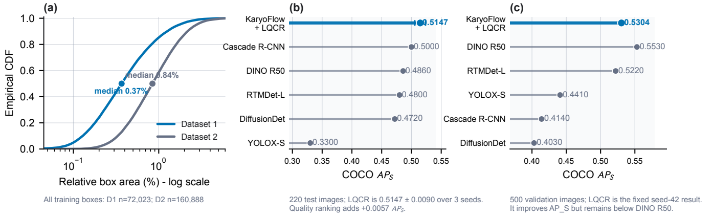
Fig. 5. Object-scale shift and small-object detection across two chromosome cohorts. (a) The empirical CDF of relative ground-truth box area over all training annotations shows that Dataset 1 chromosomes are markedly smaller than those in Dataset 2. (b) Dataset 1 test AP S is compared on 220 images; KaryoFlow+LQCR is the clean three-seed mean. (c) Dataset 2 validation AP S is compared on 500 images; LQCR is the controlled seed-42 final-only result and other detectors use unified checkpoint-linked re-evaluation. AP S is interpreted within, not across, datasets.
