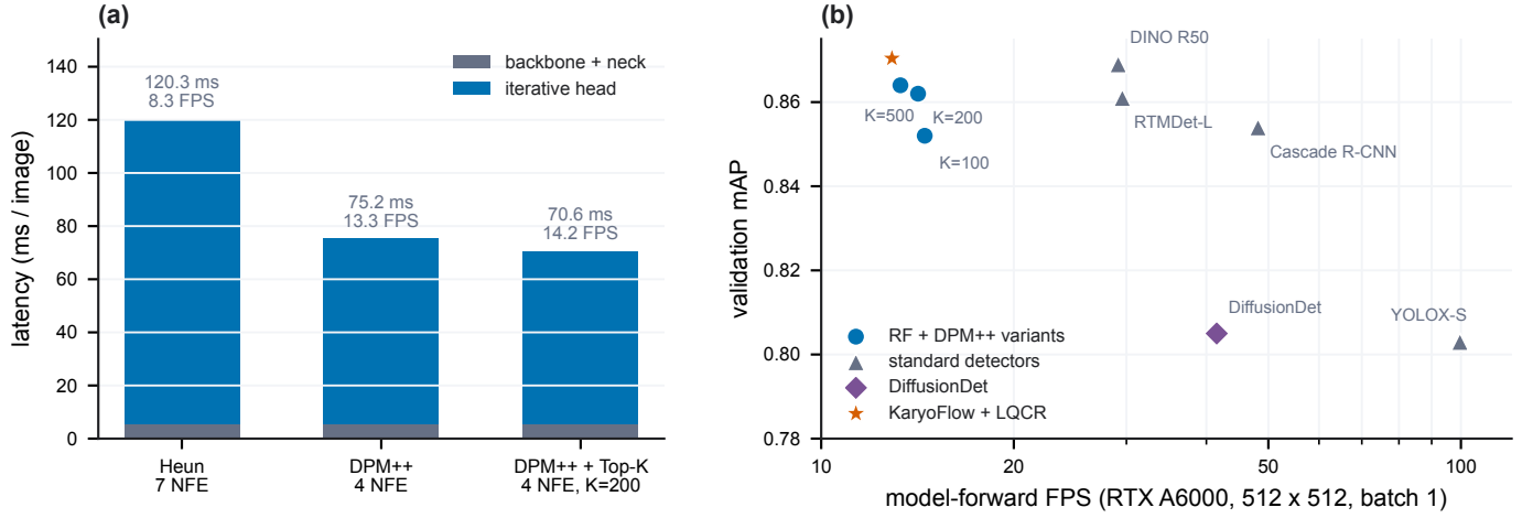
Fig. 4. Same-hardware efficiency on Dataset 2. (a) Backbone–neck and iterative-head latency are decomposed for Heun, DPM-Solver++, and proposal pruning. (b) Validation mAP is plotted against model-forward FPS on one RTX A6000. The three blue KaryoFlow operating points use K = 500 , 200, and 100 without connecting lines; the highlighted LQCR point is the complete accuracy model.
