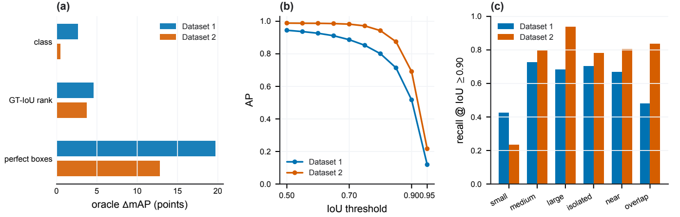
Fig. 3. Precision bottleneck diagnosis. (a) Oracle mAP headroom compares perfect classes, ground-truth-IoU ranking, and perfect coordinates; ground-truth-IoU ranking is a diagnostic upper bound, not a trained LQCR result. (b) AP is traced from IoU 0.5000 to strict localization thresholds. (c) Detection recall at IoU 0.9000 is stratified by object scale and overlap condition. Dataset 1 uses a seed-42 100-image diagnostic subset; Dataset 2 uses the seed-42 500-image validation export.
