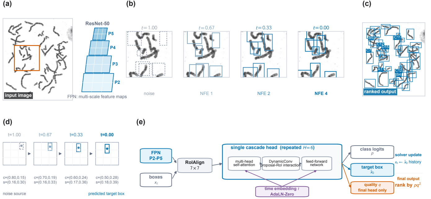
Fig. 1. KaryoFlow from image to detections. (a) A metaphase image and its ResNet-50-FPN representation provide multi-scale image features. (b) A dense crop visualizes four-NFE box refinement from noise to localized chromosome candidates. (c) The detector emits the final quality-ranked chromosome detections. (d) One proposal is shown in normalized center-and-scale coordinates along the prescribed linear RF path. (e) At each evaluation, multi-scale RoIAlign feeds a cascade head with self-attention, DynamicConv, feed-forward refinement, AdaLN-Zero time conditioning, and the final-head quality branch. Endpoints and output boxes are empirical; intermediate boxes visualize the prescribed RF path rather than recorded hidden activations.
