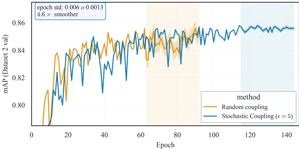
Training Stability: Random vs Stochastic Coupling
