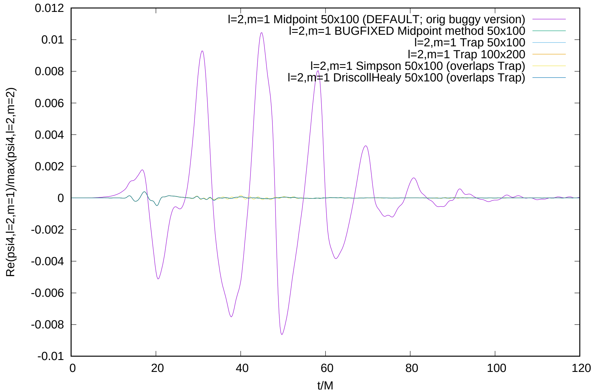
QC-0 BBH l=2, m=1 (spin-weight -2 sph. harm.) mode of \text{Re}(\psi_4)
