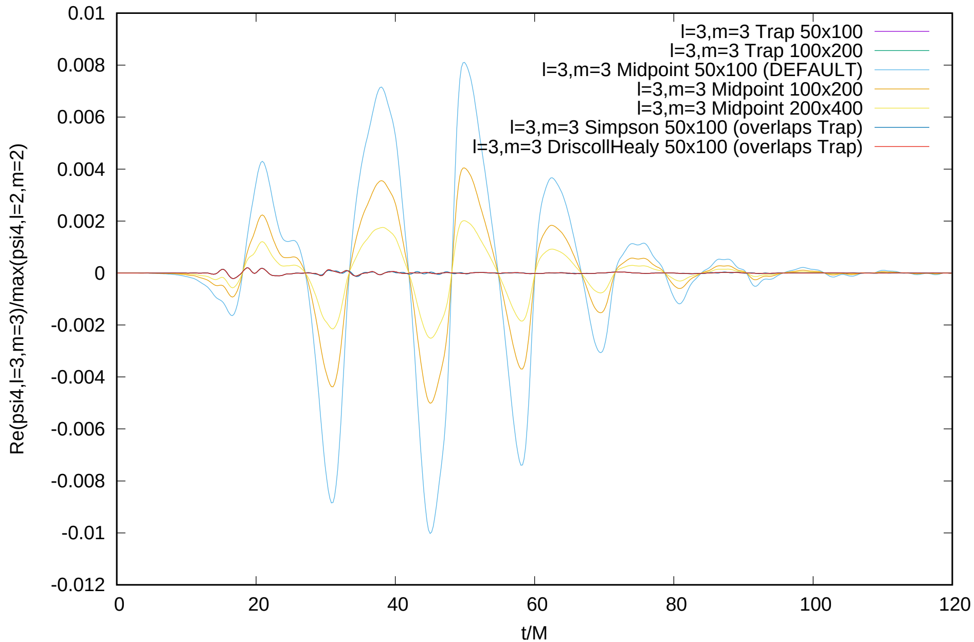
QC-0 BBH l=3, m=3 (spin-weight -2 sph. harm.) mode of \text{Re}(\psi_4)
