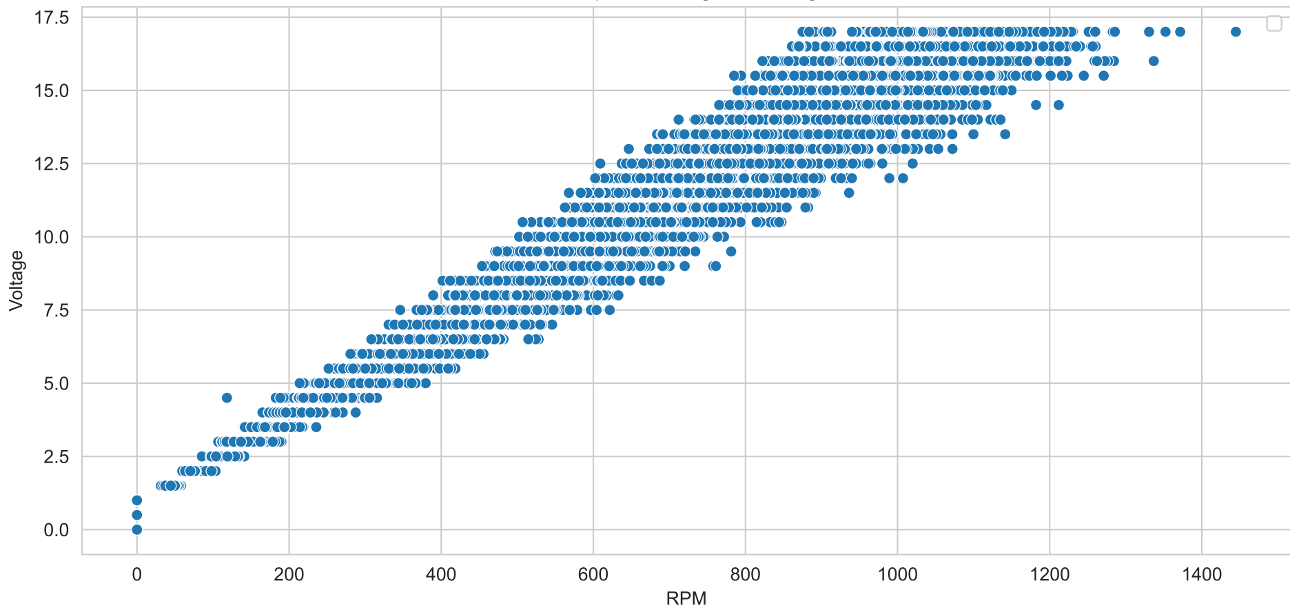
Data points using back-EMF.
