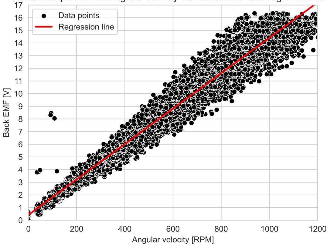
Relationship Between Angular Velocity and Back-EMF with regression line.
