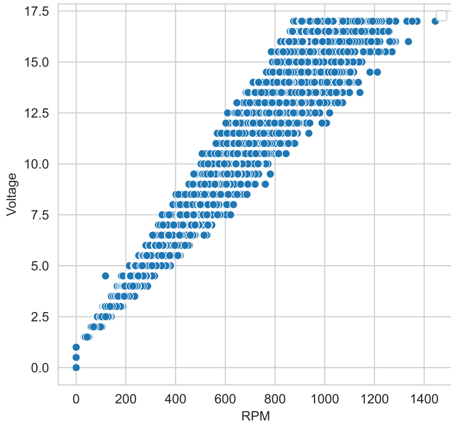
Data points using bus voltage
