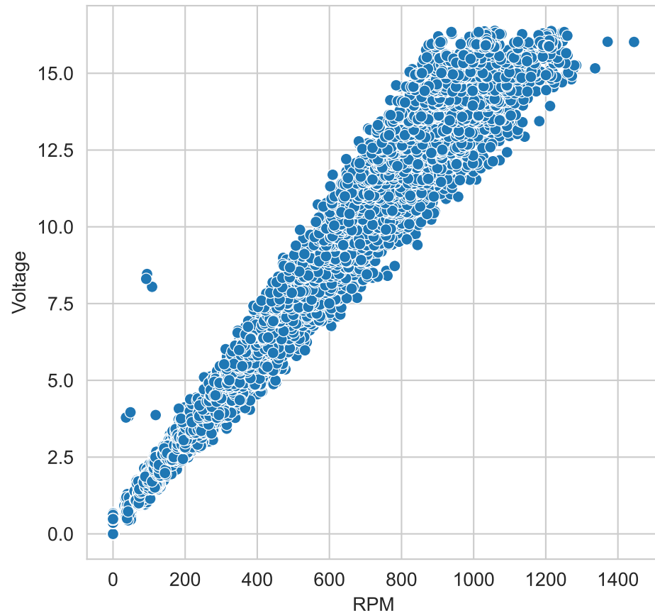
Data points using back-EMF.
