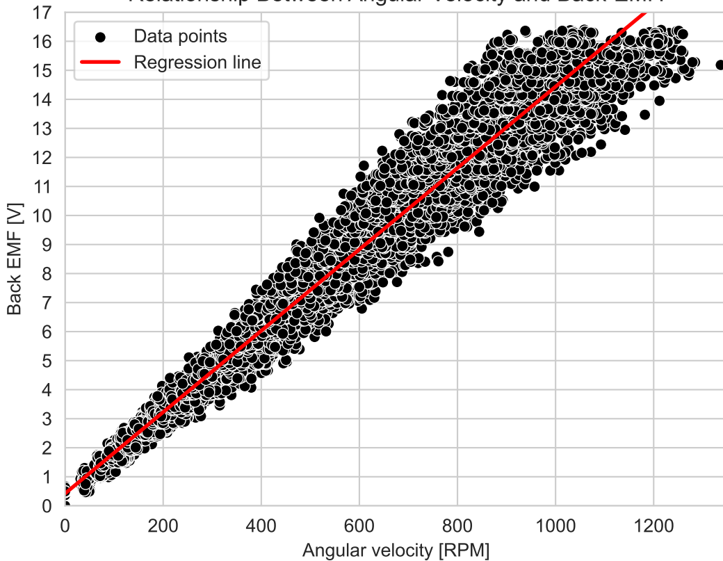
Relationship Between Angular Velocity and Back-EMF.
