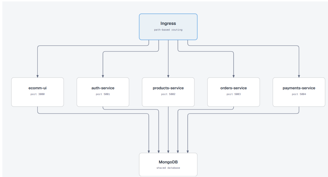
Figure 4.2: Application-layer access structure. The Ingress routes by path to ecommm-ui and each of the four backend services by their internal ClusterIP service name and port; every workload, including ecommm-ui itself, holds its own connection to the single shared MongoDB instance.
