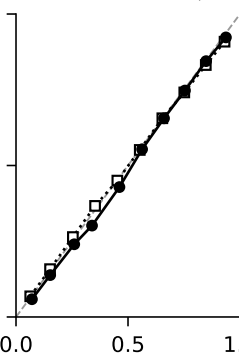
ASSISTments-2009, DKT
