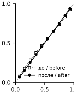
ASSISTments-2012, AKT
