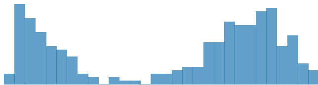
Old Faithful geyser (N=272)
