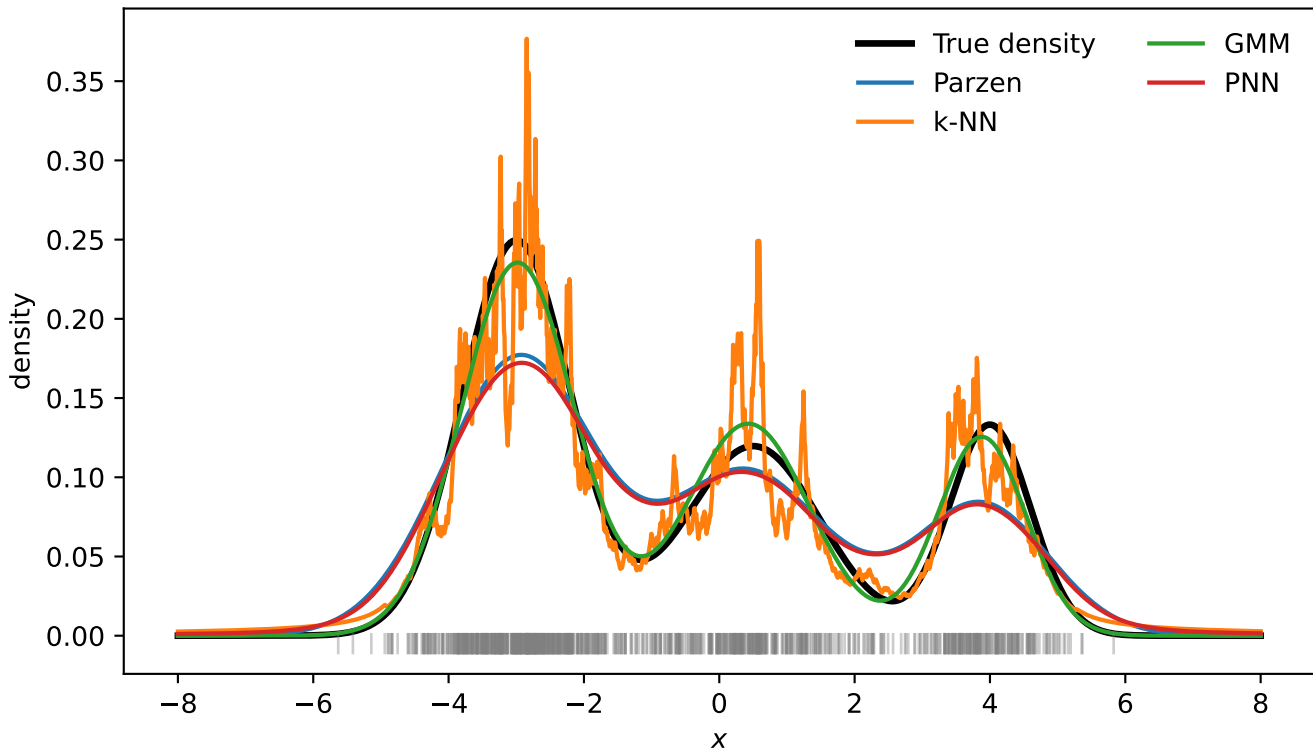
1D synthetic: true density vs estimators
