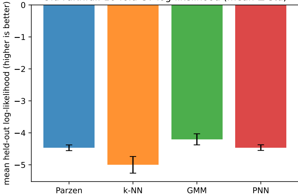
Old Faithful: 10-fold CV log-likelihood (mean \pm std)
