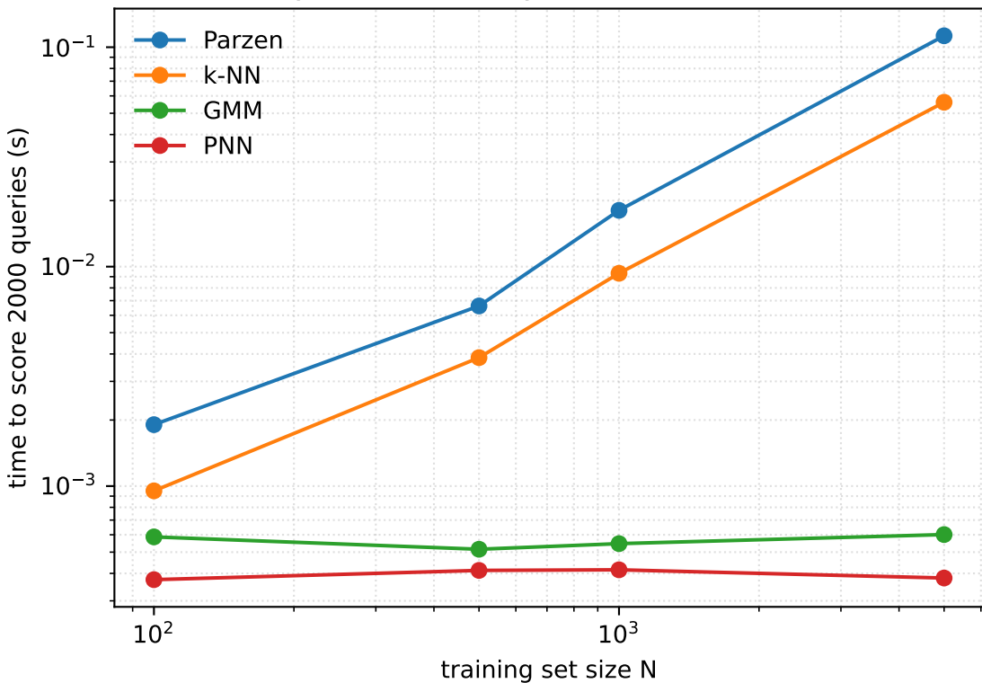
Query-time scalability: PNN is \sim constant in N
