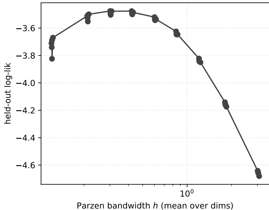
Parzen: bandwidth vs log-likelihood
