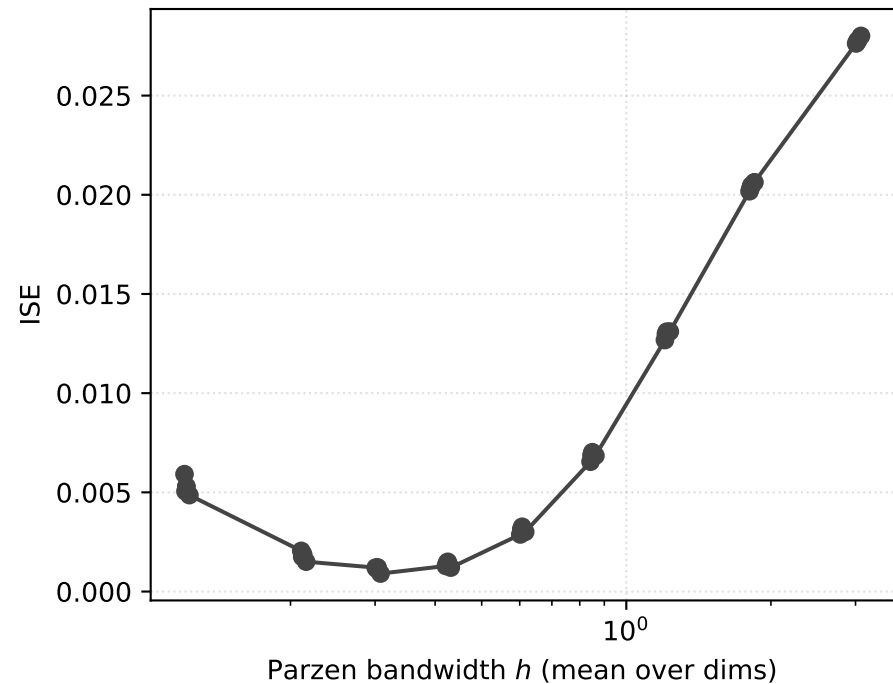
Parzen: bandwidth sensitivity
