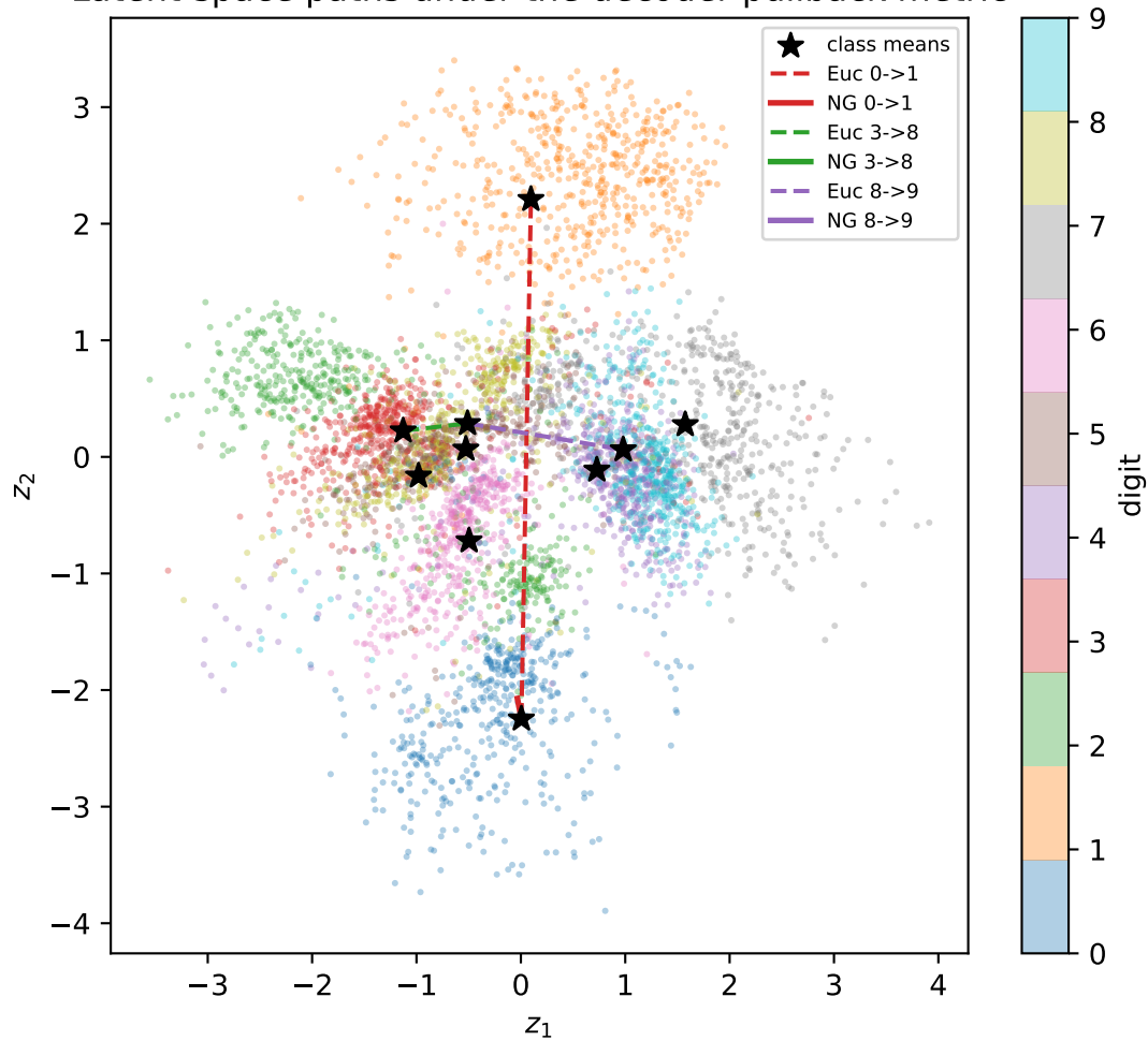
Latent-space paths under the decoder pullback metric
