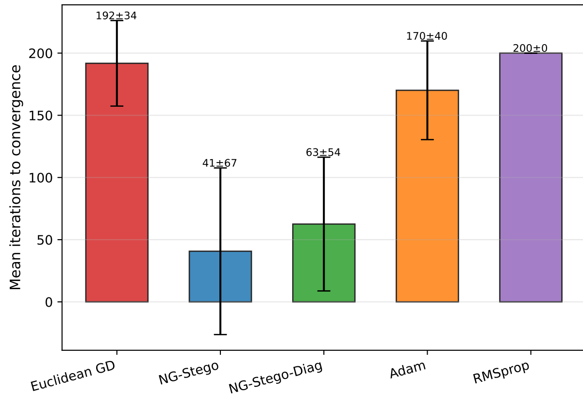
Convergence comparison (non-diagonal FIM, N=20 runs)
