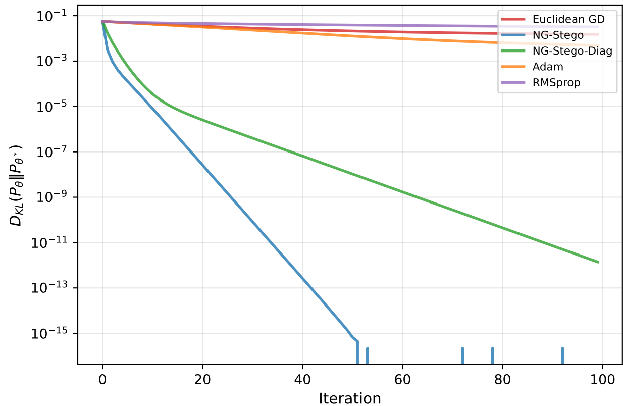
KL convergence trajectory (representative run)
