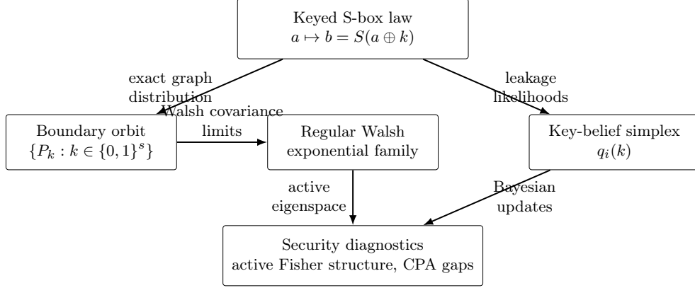
Fig. 1 Boundary-to-belief framework. The exact keyed S-box laws lie on a singular boundary orbit, the Fisher calculations are made in a regular Walsh exponential family or in boundary covariance limits, and CPA updates evolve on the separate key-belief simplex.
