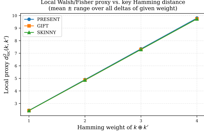
Fig. 5 Local proxy versus key-difference Hamming weight. The plot aggregates the same covariance-weighted Walsh displacement by the Hamming weight of k \oplus k' ; it is not an exact Fisher–Rao distance between the singular distributions.
