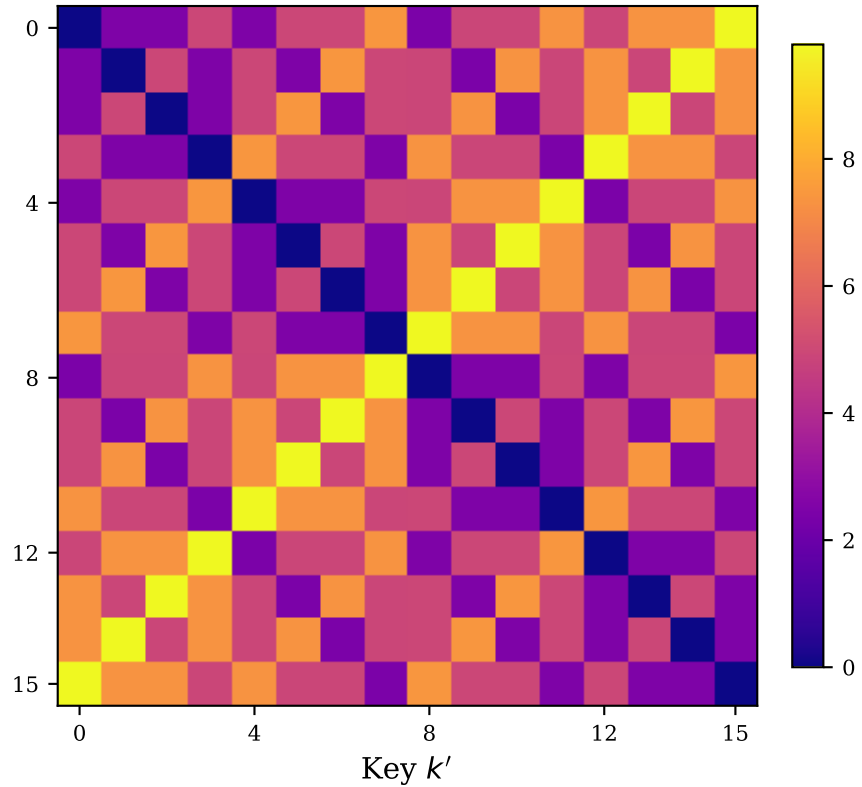
PRESENT
