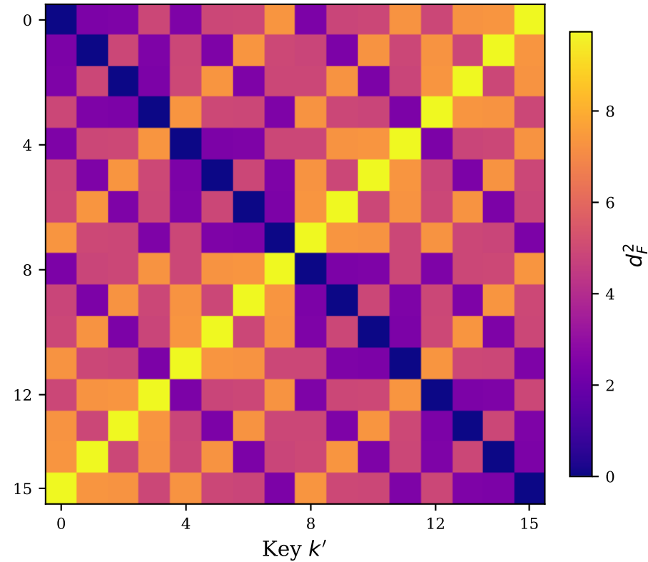
SKINNY
