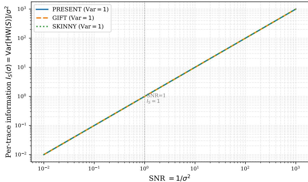
Per-trace Fisher information (Hamming weight model)
