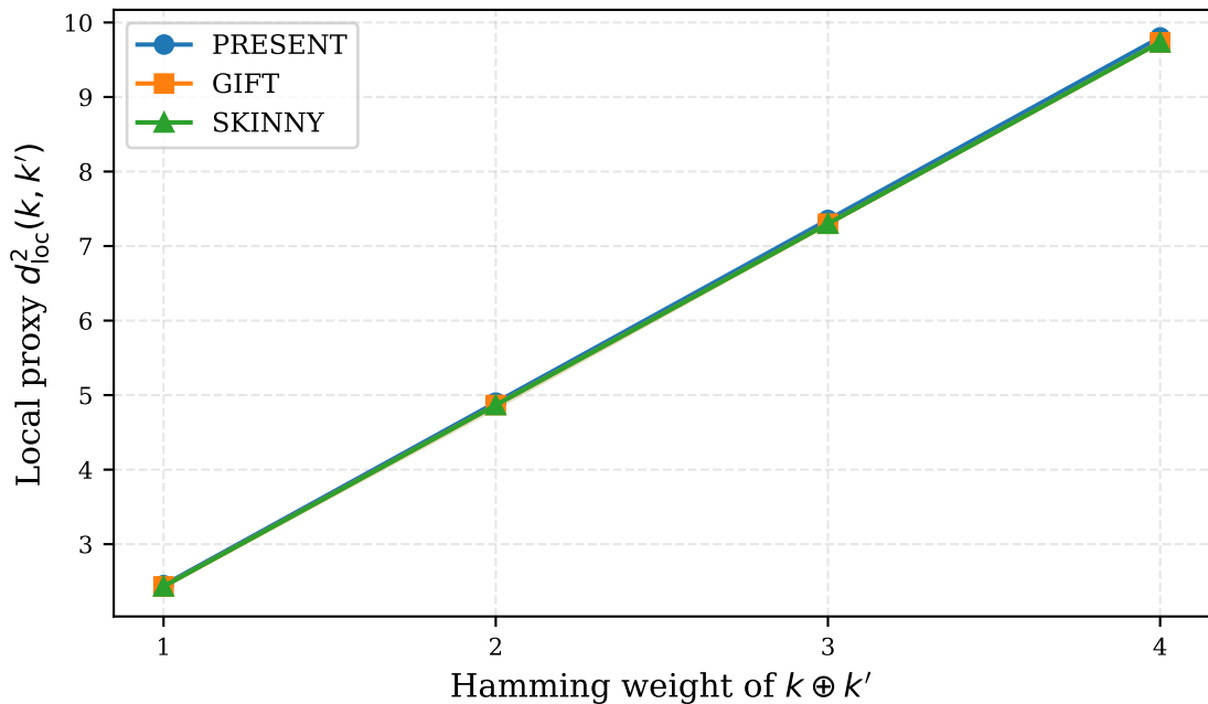
Local Walsh/Fisher proxy vs. key Hamming distance (mean \pm range over all deltas of given weight)
