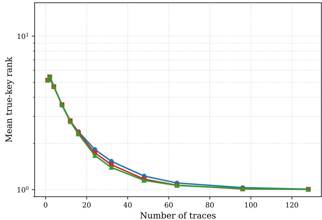
Simulated CPA under Hamming-weight Gaussian leakage (sigma=2, 3000 trials, seed=20260622)
