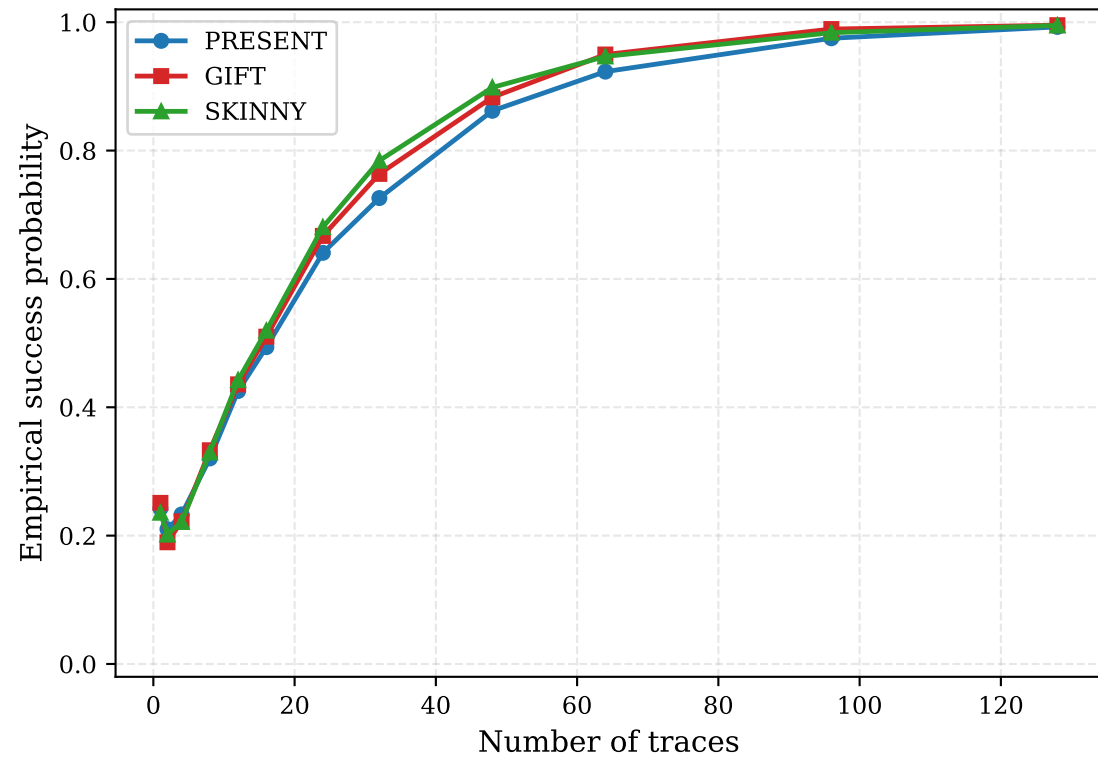
Simulated CPA under Hamming-weight Gaussian leakage (sigma=2, 3000 trials, seed=20260622)
