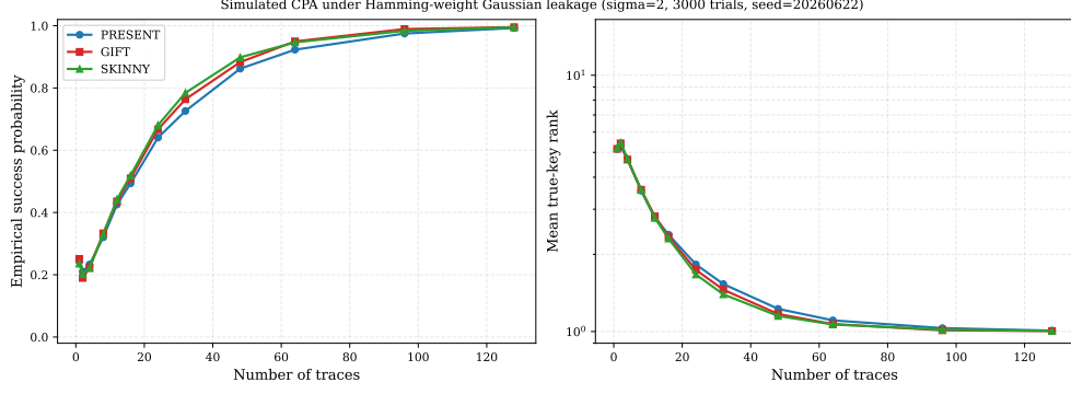
Fig. 6 Simulated CPA under Hamming-weight Gaussian leakage. The left panel shows empirical success probability and the right panel shows mean true-key rank over 3000 trials. The curves translate the pairwise-gap analysis into trace-dependent attack observables.
