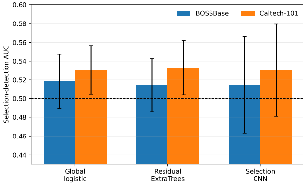
Figure 6: Mean selection-detection AUC and 95% Student- t intervals over five partitions per dataset. The dashed line denotes chance performance.
