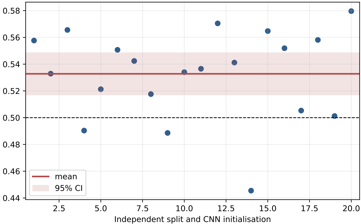
Selection-detection AUC
