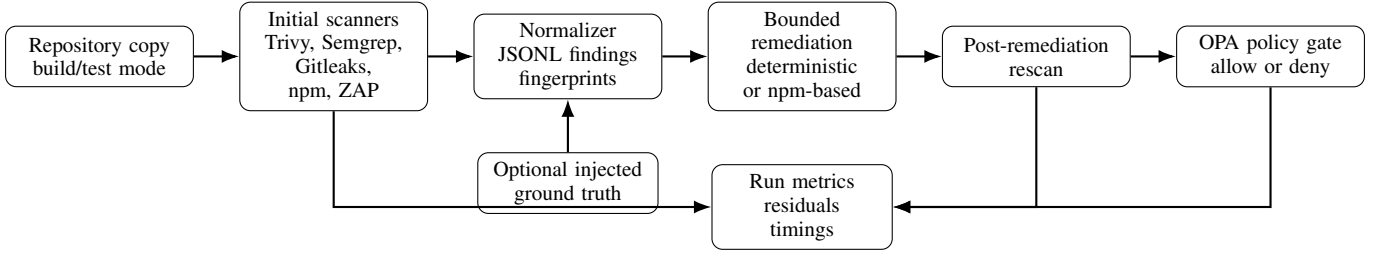
Fig. 1. SecFlowOps workflow and measurement architecture. Scanners produce normalized findings, bounded remediators edit only the copied workspace, a second scanner pass measures residual findings, and OPA decides whether the residual state satisfies the delivery policy.
