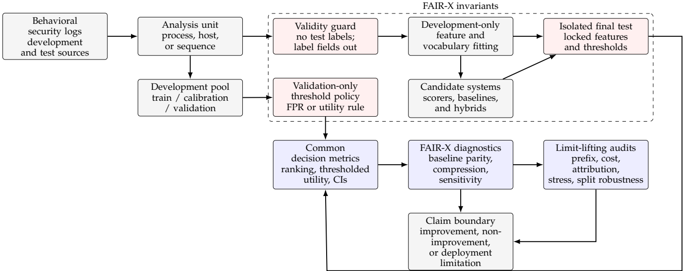
Fig. 1. General FAIR-X threshold-transfer evaluation contract. Red blocks are non-negotiable validity guards; blue blocks are audits that determine whether a performance claim, negative result, or deployment boundary is defensible. FAIR-BETH instantiates this contract for process-level BETH evaluation.
