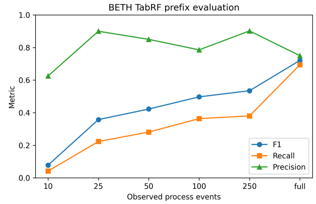
Fig. 9. BETH TabRF prefix curve. Unlike MalBehavD-V1, BETH requires much more of the process trace before recall becomes useful.
