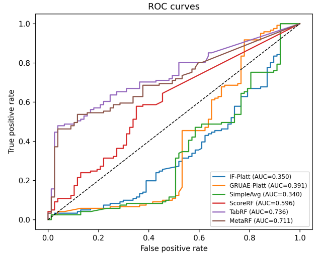
Fig. 2. ROC curves on the official BETH test split. The tabular and meta Random Forests have stronger ranking behavior than the raw detector scores.
