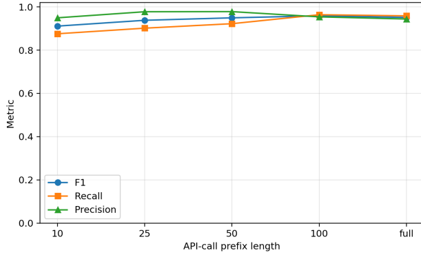
Fig. 6. MalBehavD-V1 prefix evaluation. The curve shows that useful discrimination is available before the full API-call sequence is observed.
