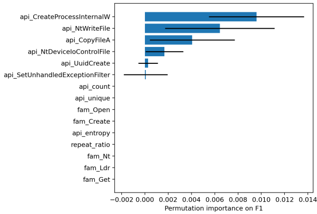
Fig. 7. Permutation feature importance on MalBehavD-V1. Attribution is computed after final evaluation and is used only for interpretation.
