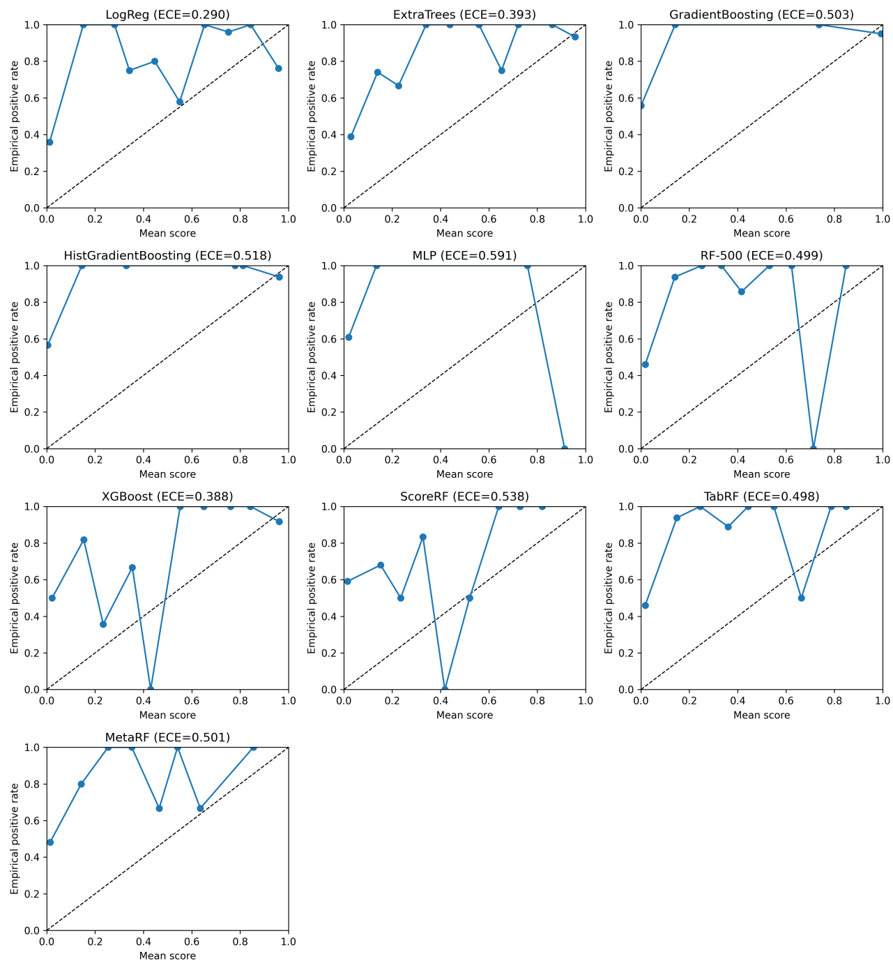
Fig. S1. Reliability diagrams on the official BETH test split. These curves support score-and-threshold language rather than posterior-risk language.
