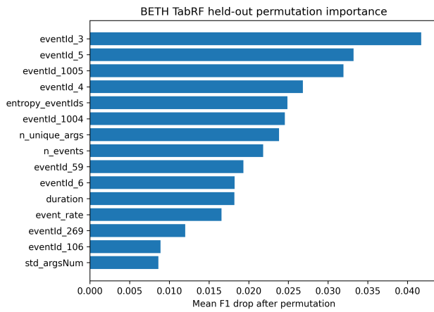
Fig. S3. Held-out permutation importance for BETH TabRF.
