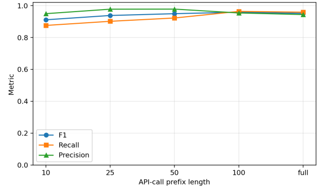
Fig. 5. MalBehavD-V1 prefix evaluation. The curve shows that useful discrimination is available before the full API-call sequence is observed.
