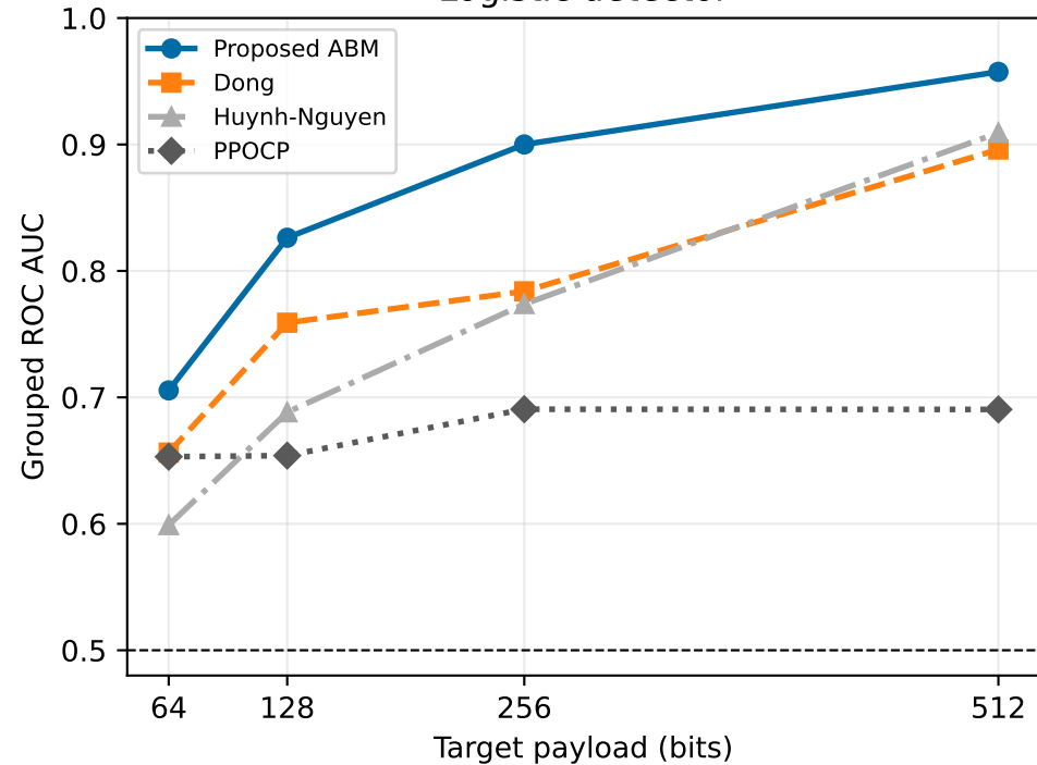
Logistic detector
