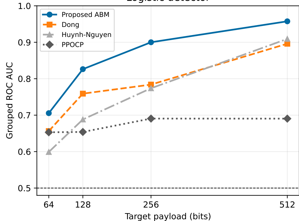
Logistic detector
