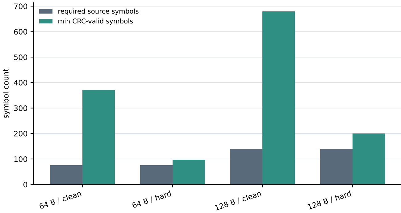
Exact recovery margin on the public VQGAN checkpoint
