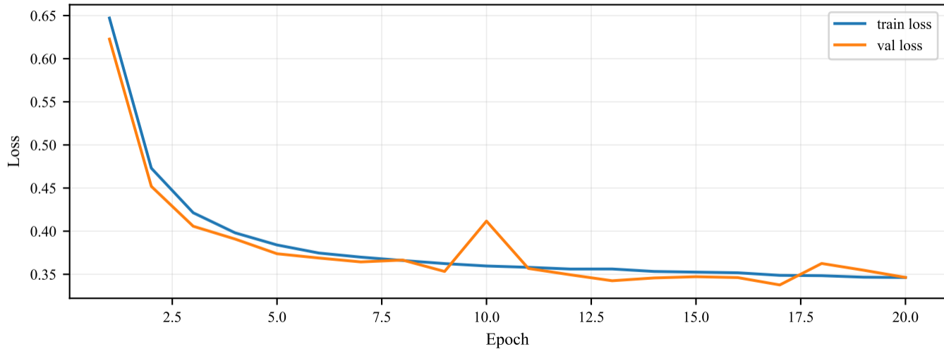
Training Curves — Loss
