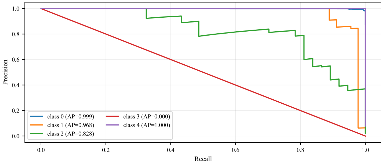
Precision–Recall Curves (One-vs-Rest)
