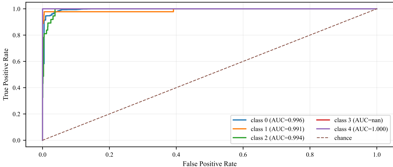
ROC Curves (One-vs-Rest)
