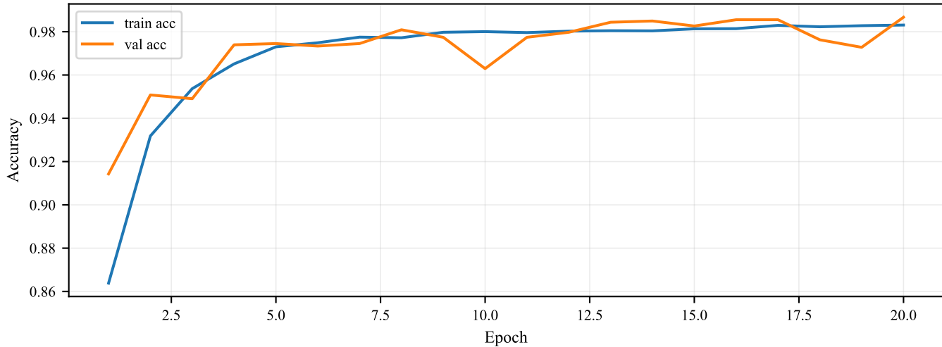
Training Curves — Accuracy
