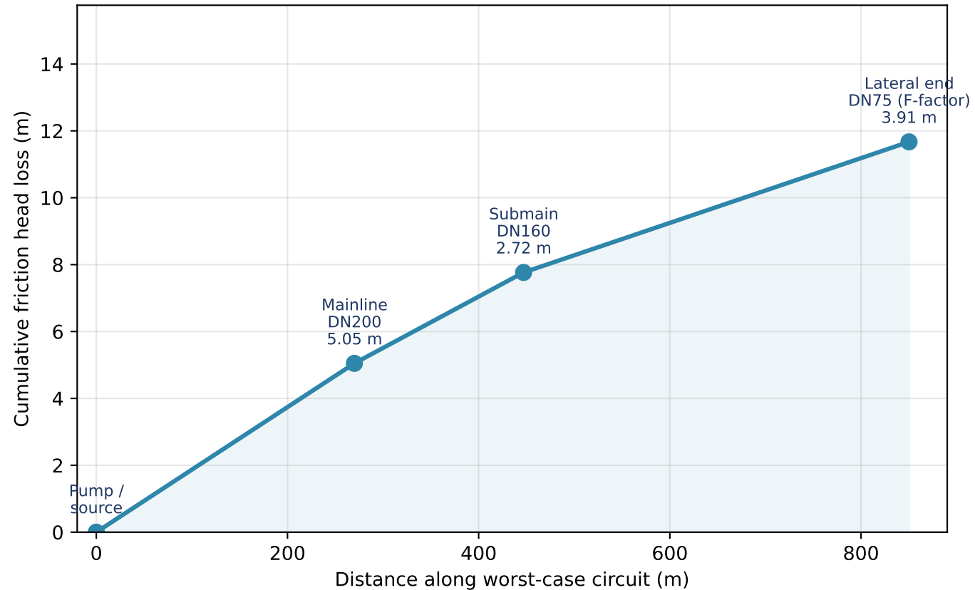
Hydraulic head-loss profile along the worst-case circuit (Hazen-Williams C = 150; total \approx 11.67 m)
