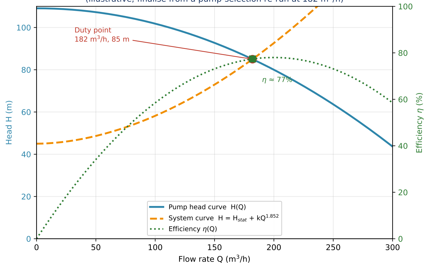
Pump head-flow and system curves, duty at the 182 m 3 /h peak (illustrative; finalise from a pump-selection re-run at 182 m 3 /h)
