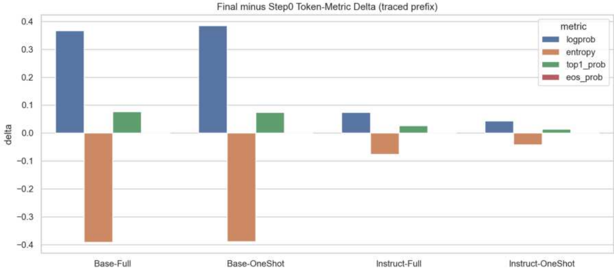
Figure 18: Token-level deltas from the initial to final checkpoint.
