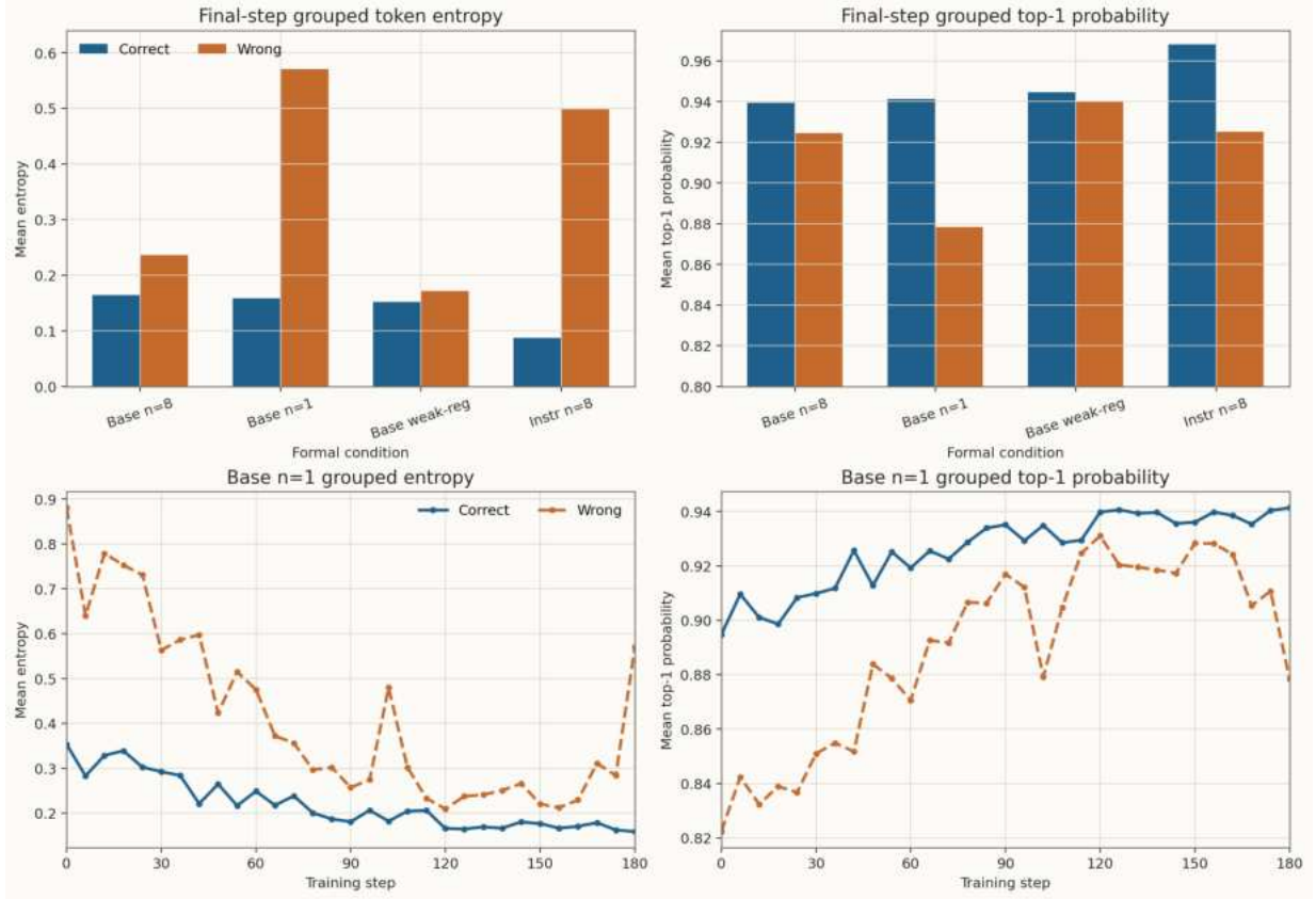
Figure 19: Correctness-conditioned token-distribution statistics. The top row compares final-checkpoint correct and wrong responses; the bottom row tracks the same grouped statistics over training for Base n=1 .
